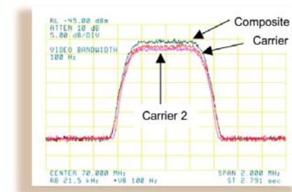
Figure 2: Duplex Link with DoubleTalk Carrier-in-Carrier
