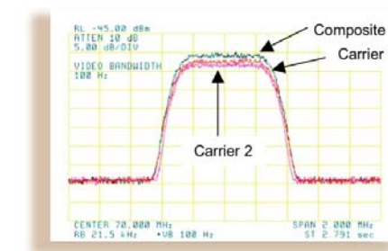
Figure 2: Duplex Link with DoubleTalk Carrier-in-Carrier
