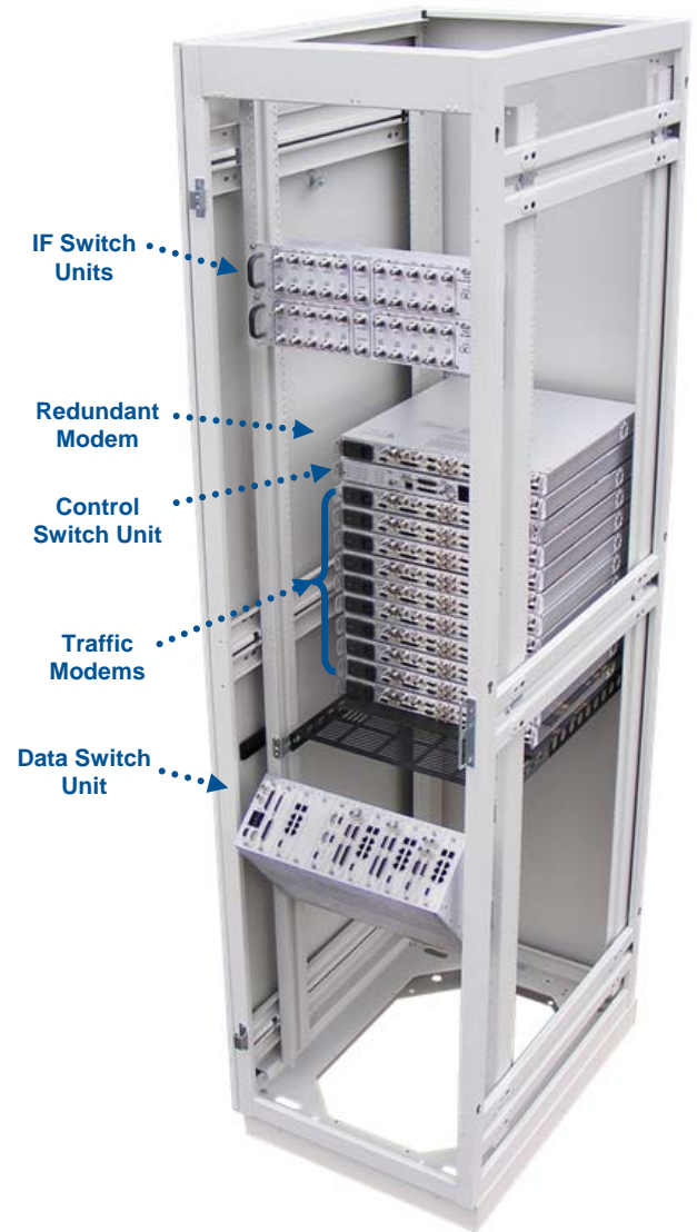
CRS-500 1:N Modem Redundancy System Typical Rack View (back side)
