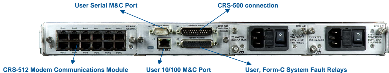
Control Switch Unit (CSU) – Rear View
