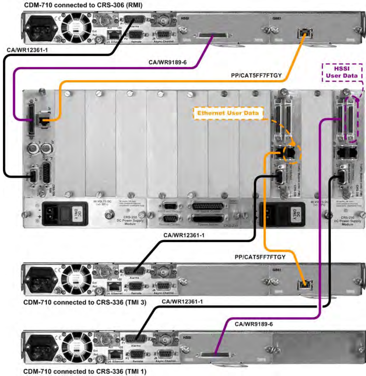
Figure 4-29. Control and Data Cables Example #2 – CRS-300 to CDM-710 (Connections shown for RMI & TMIs 1 and 3 only)
