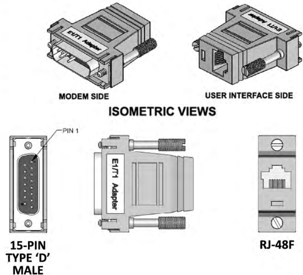
Figure B-28. Optional T1/E1 Adapter (CN-0000268)
