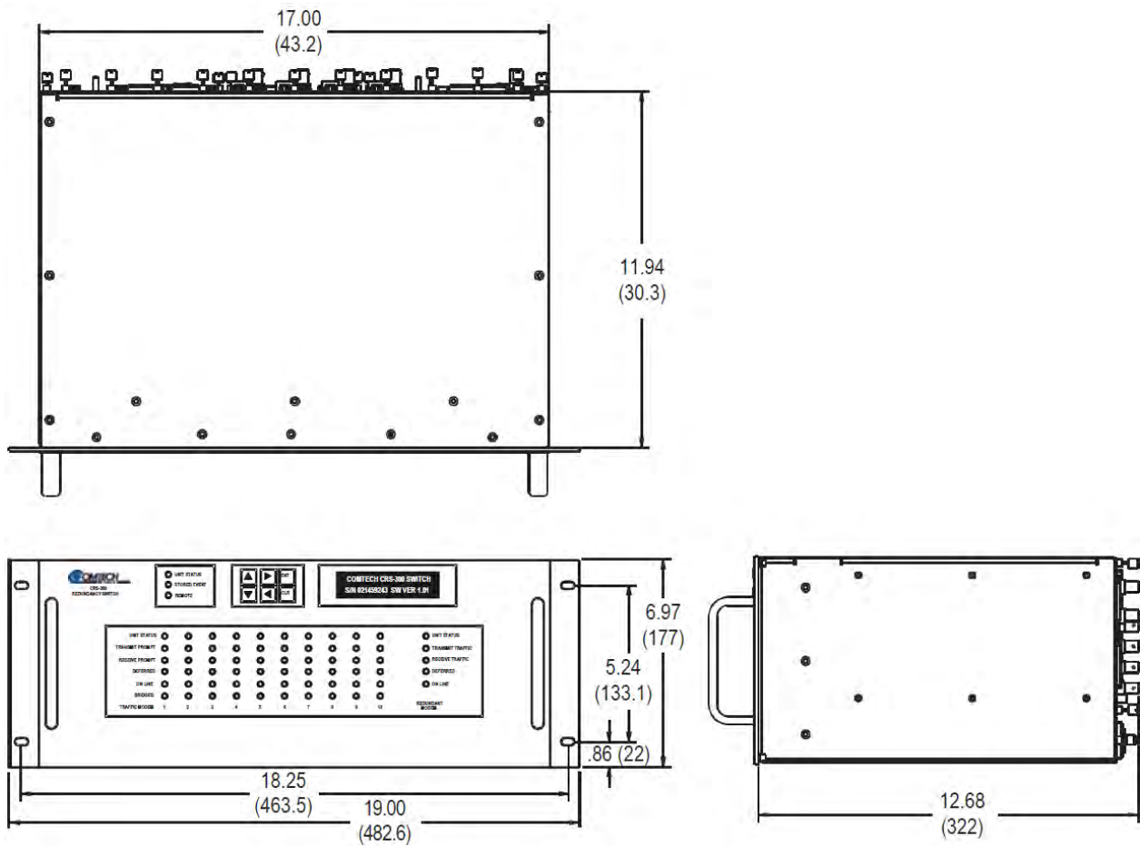
Figure 1-27. CRS-300 1:1 Redundancy Switch
