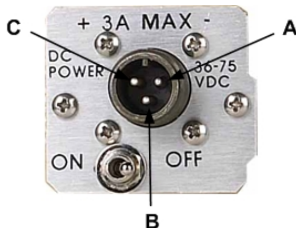
Figure 5-1. DC Power Input and Switch
